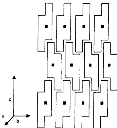
Figure 14. Schematic representation of the two-dimensional array [(100) plane] of interdigitated (salicylaldiminato)copper complexes 53 in the S_A phase. (Reprinted from ref 75. Copyright 1991 American Chemical Society.)
