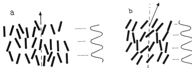
Figure 2. (a) Schematic representation of a smectic A ( S_A ) calamitic phase and (b) schematic representation of a smectic C ( S_C ) calamitic phase.
