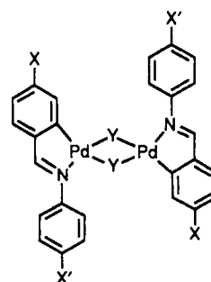
22a: Y = CH 3 COO, X = H, Me, OMe, Cl, CN, NO 2 , X' = OC 8 H 17 b: Y = CH 3 COO, X' = H, Me, OMe, Cl, CN, NO 2 , X = OC 8 H 17 c: Y = Cl, X = H, Me, OMe, Cl, CN, NO 2 , X' = OC 8 H 17 d: Y = Cl, X' = H, Me, OMe, Cl, CN, NO 2 , X = OC 8 H 17 e: Y = Cl, X = H, Me, OMe, Cl, CN, NO 2 , X' = OC 8 H 17 f: Y = Cl, X = H, OC 2 H 5 , OC 8 H 13 , OC 10 H 21 , X' = OC 10 H 21
