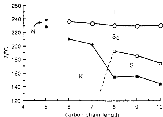
Figure 4. Phase diagram for nickel bis[4-(alkoxy)dithiobenzoates] 8. The symbols are as follows: ●, K–N; ◆, K–S C ; ◇, N–I; ■, K–S X ; □, S X –S C ; ○, S C –I.
