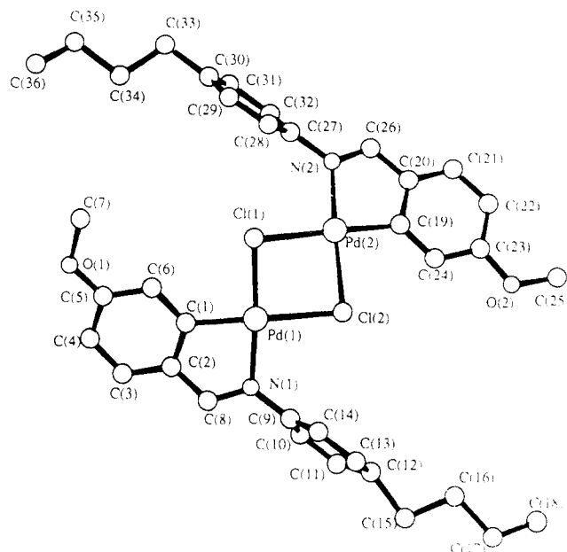
Figure 9. Single-crystal X-ray structure of the mesogenic cyclopalladated complex 24. (Reprinted from ref 36. Copyright 1990 Taylor & Francis.)
