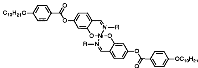
7: R = C 5 H 11 , C 10 H 21 , C 6 H 4 OMe
