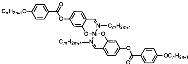
5: m = 1, n = 8, 11, 14 m = 13, n = 12
