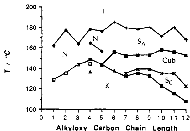
Figure 16. Polymorphism exhibited by the bis[4-(alkyloxy)silbazole]silver dodecyl sulfates 59. Symbols are as follows: \square , K-N; \diamond , N-I; \square , K-SA; \diamond , SA-N; \blacksquare , (SA-SC); \square , (SA-NR); \triangle , (NR-SC); \triangle , K-Cub; \square , Cub-SA; + , SA-I; \boxtimes , K-SC; \times , SC-Cub.
